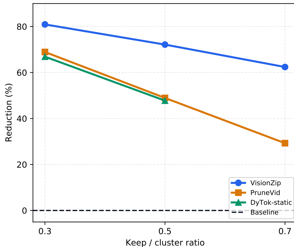
Token Reduction vs Baseline
