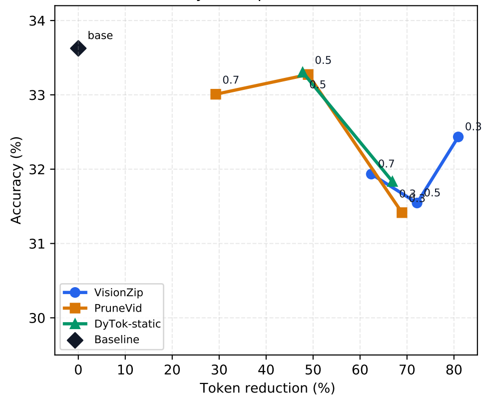
Accuracy / Compression Trade-off
